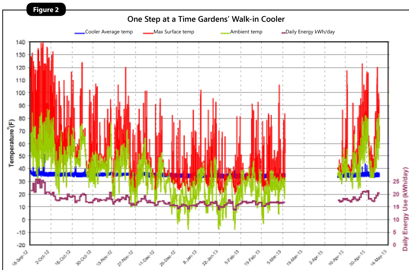
Figure 2. Average daily internal cooler temperature, maximum external cooler surface temperature, ambient air temperature and daily energy use for the walk-in cooler at One Step at a Time Gardens from Sept. 18, 2012 – May 7, 2013. The gap in data corresponds to a data-logging system malfunction.
